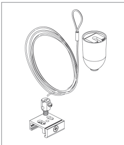
Suspension kit with brackets
