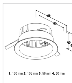
Recessed case for surface accessories
