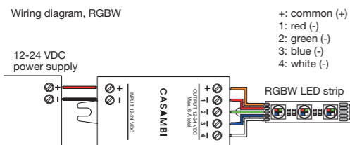
Wiring diagram, RGBW
