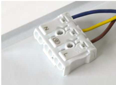
Quick connector.
